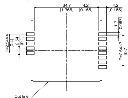
Recommended measurements for mounting board (SMD type)
