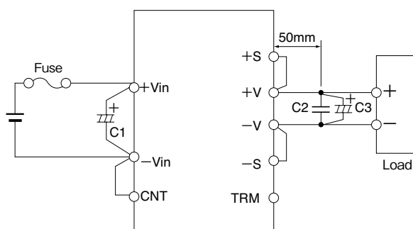
Fig.1-2 Basic Connection
