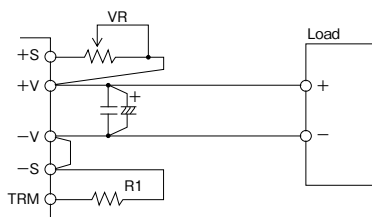
Fig.2-5 Example connection of external resistor
