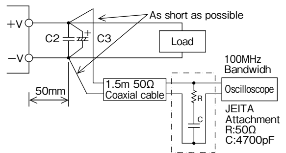
Fig.3-1 Measurement of Maximum Output Ripple & Noise Based on JEITA RC-9141
