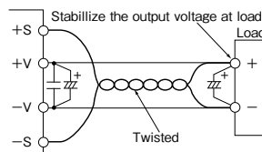
Fig.9-1 Remote Sensing in Use
