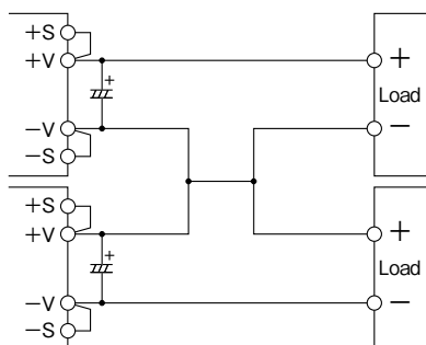
Fig.12-2 ±Output Series Operation
