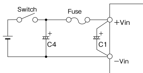
Fig.1-3 Input filter (C4) with Switch
