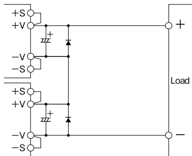
Fig.12-1 Series Operation for High Output Voltage Application
