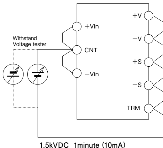
Fig.19-1 Withstand Voltage Test for Input-Output
