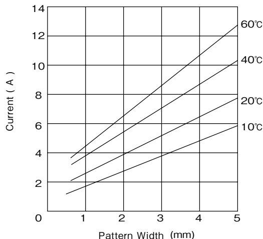
Fig.2-2 Characteristic of current allowance
