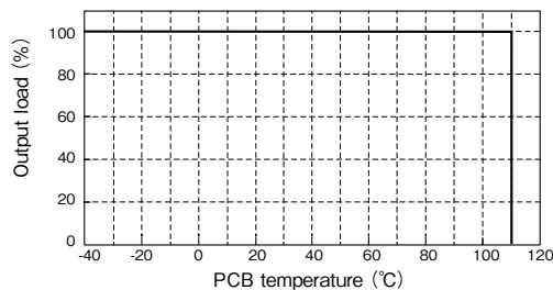
Fig.1-12 Output Derating by PCB Temperature
