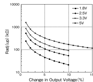
Fig.2-4 Δ (%) vs. R adj (up)
