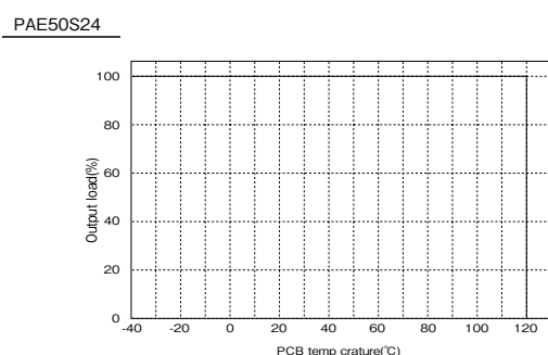
Fig.1-5 Output Derating by PCB Temperature
