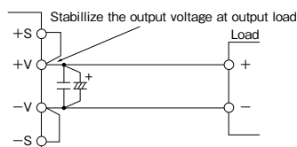
Fig.9-2 Remote Sensing Not in Use (Local Sensing)
