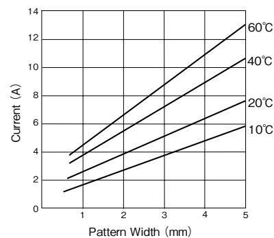
Fig.2-2 Characteristic of current allowance
