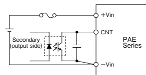
Fig.10-1 CNT connection
