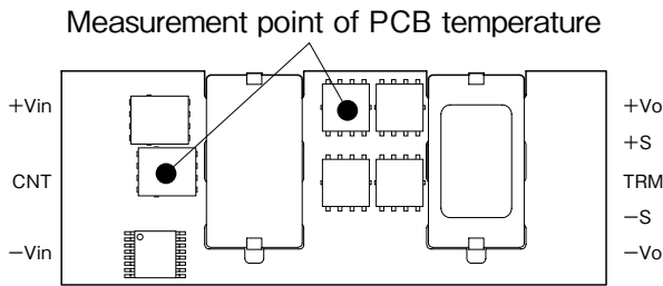
Fig.1-4 Measurement point of PCB temperature
