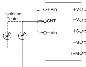
Fig.20-1 Isolation test
