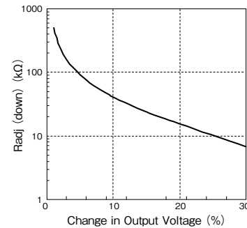
Fig.2-2 Δ (%) vs. R adj (down)
