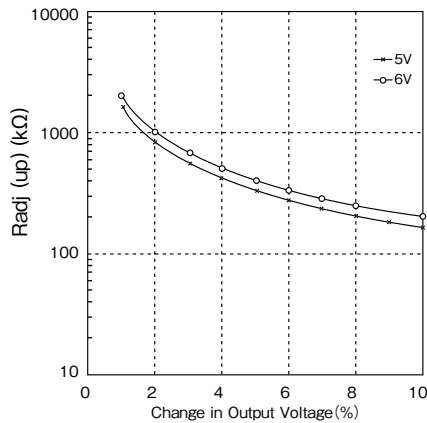
Fig.2-4 \Delta(\%) vs. R_{adj}(up)
