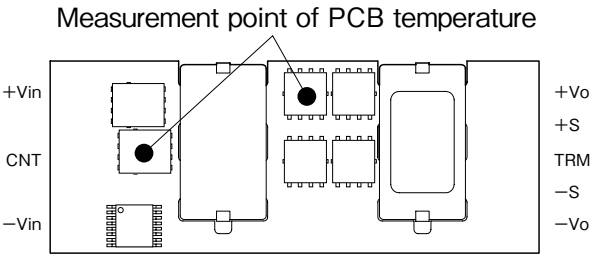
Fig. 1-11 Measurement point of PCB temperature
