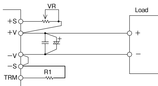
Fig.2-5 Example connection of external resistor
