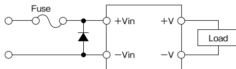
Fig.1-5 Protection for Reversed Input Connection
