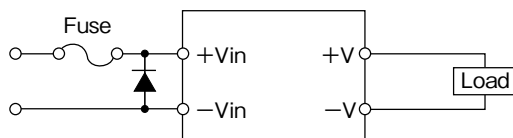
Fig.1-5 Protection for Reversed Input Connection
