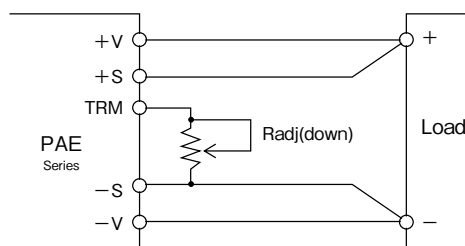
Fig.2-1 Connection for output voltage trim down
