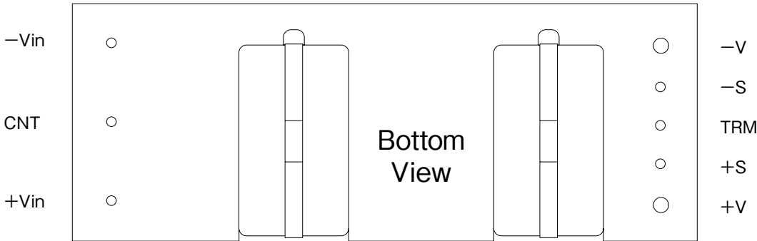
Input and Output Terminal Configurations (Bottom View)
