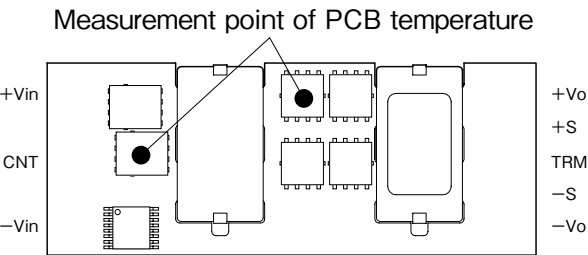
Fig. 1-11 Mesurement point of PCB temperature
