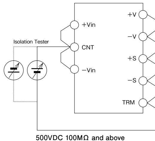
Fig.20-1 Isolation test
