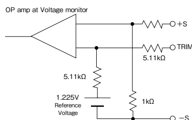
Fig.2-6 Trim circuit composition
