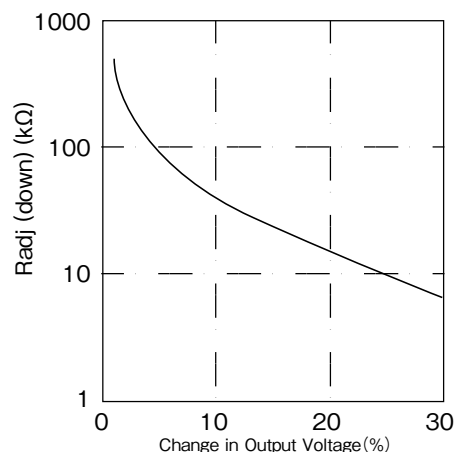
Fig.2-2 \Delta(\%) vs. Radj (down)
