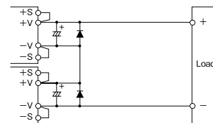
Fig.12-1 Series Operation for High Output Voltage Application
