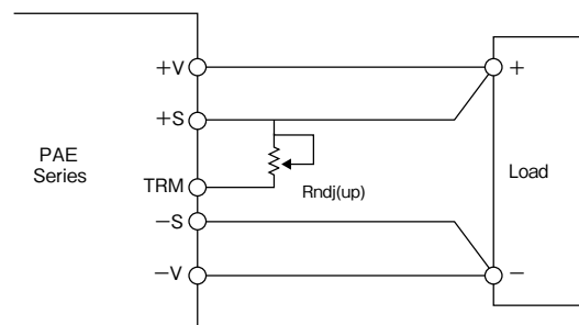
Fig.2-3 Connection for output voltage trim up
