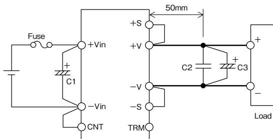
Fig.1-2 Basic Connection
