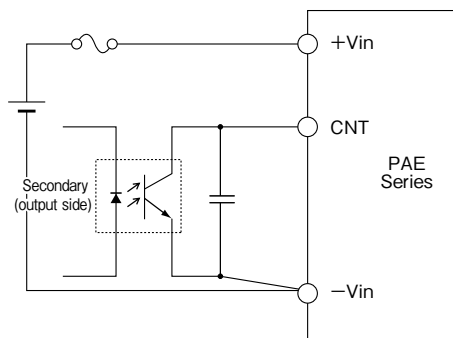
Fig.10-1 CNT connection
