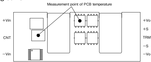
Fig.1-11 Measurement point of PCB temperature
