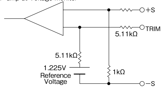
Fig.2-6 Trim circuit composition
