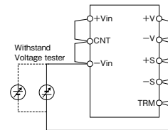
Fig.19-1 Withstand Voltage Test for Input-Output
