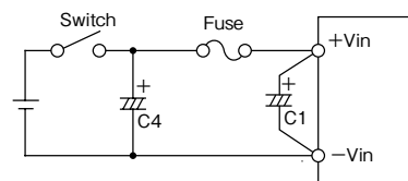
Fig.1-3 Input filter (C4) with Switch
