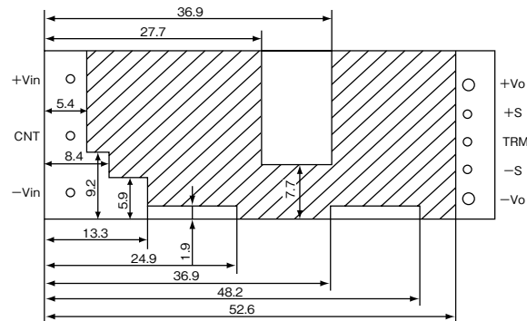
Fig.2-1 Prohibition area of wiring pattern
