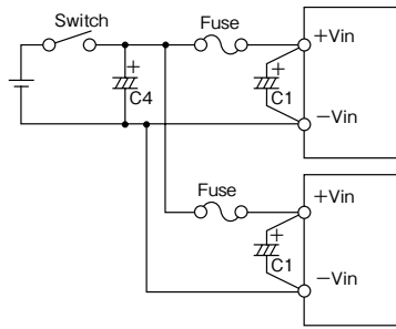
Fig.1-4 Input Filter with Switch when Plural Power Modules are connected
