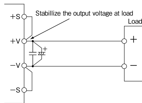
Fig.9-2 Remote Sensing Not in Use (Local Sensing)
