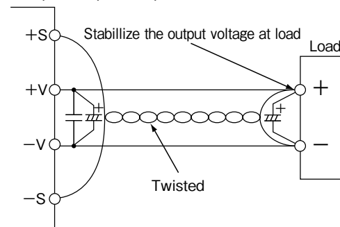
Fig.9-1 Remote Sensing in Use
