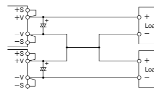
Fig.12-2 ±Output Series Operation
