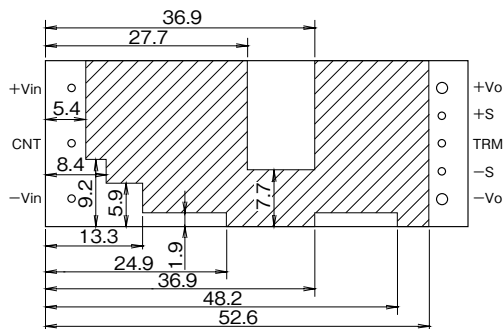
Fig.2-1 Prohibition area of wiring pattern
