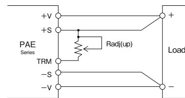
Fig.2-3 Connection for output voltage trim up
