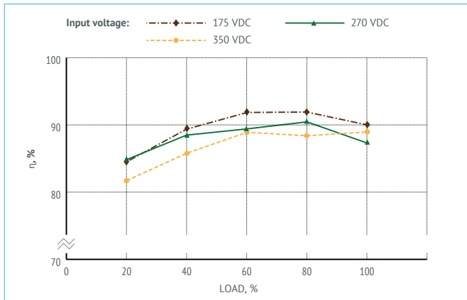
Figure 5. Efficiency of MDVHx400-1M28.
