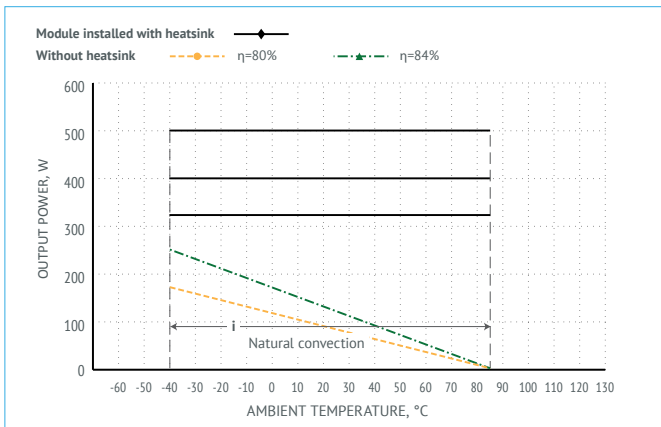
Figure 6 (a). Power derating of MDVHi500.
