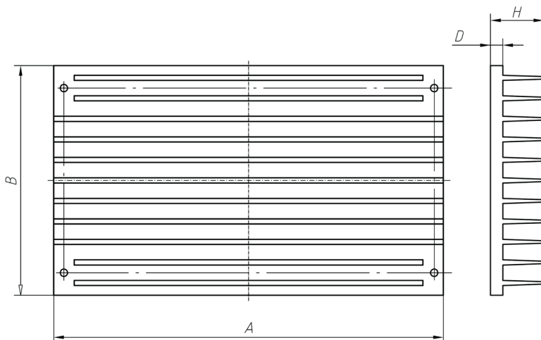
Figure 10. Heatsink with longitudinal ribs for index "i" – 122×82×14×6 mm and index "m" – 122×82×24×6 mm (A×B×H×D).
