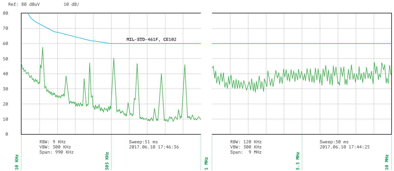
Figure 8. Spectrogram of MDVH500-1M28 with typical connection diagram.
