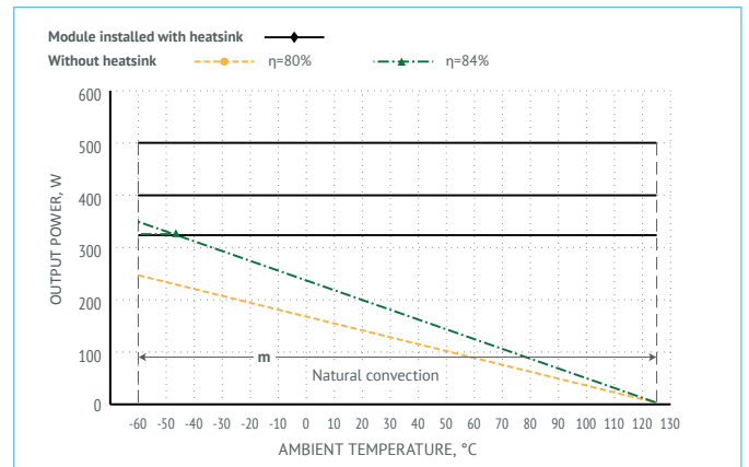
Figure 6 (b). Power derating of MDVHm500.
