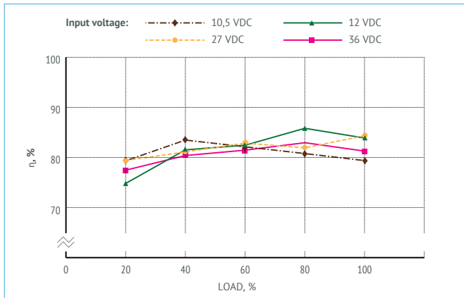
Figure 6 (a). Efficiency of MDVx50-1B05.
