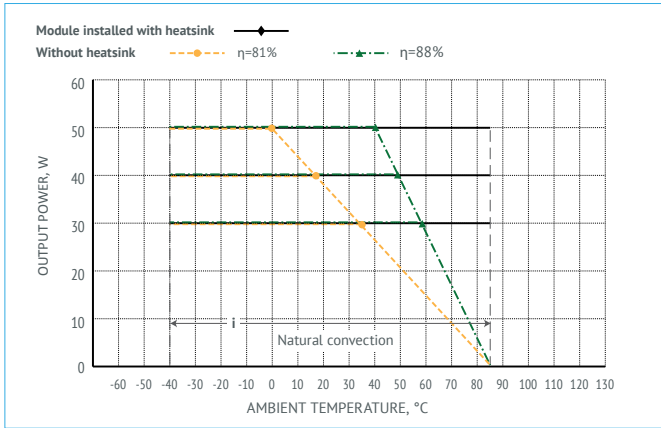
Figure 7 (a). Power derating of MDVi50-xxx.
