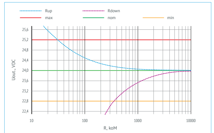
Figure 5 (d). Current and voltage values for adjustment of MDVx50-xx24.
