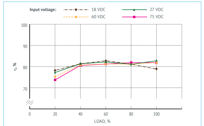
Figure 6 (b). Efficiency of MDVx50-1W05.
