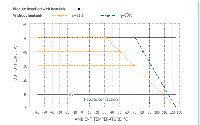
Figure 7 (b). Power derating of MDVm50-xxx.
