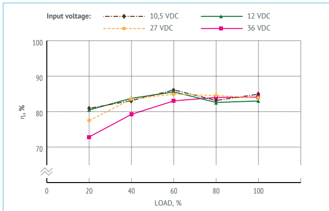
Figure 6 (c). Efficiency of MDVx50-1B27.
