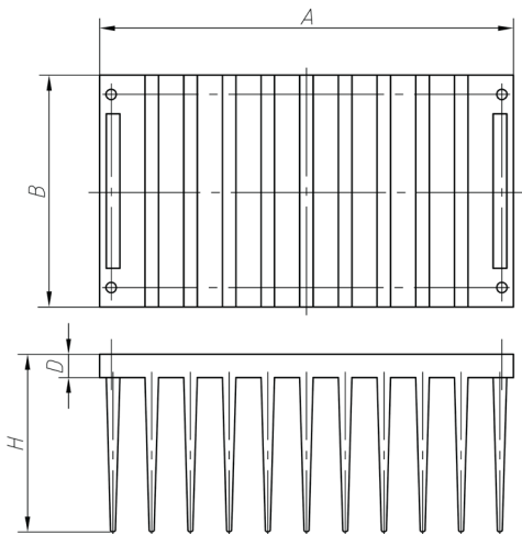
Figure 11 (a). Heatsink with transversal ribs for index "i" – 67,5×40×14×4 mm and index "m" – 67,5×40×24×4 mm (A×B×H×D).
