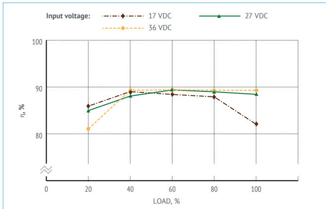
Figure 5. Efficiency of MDVx160-1V27.
