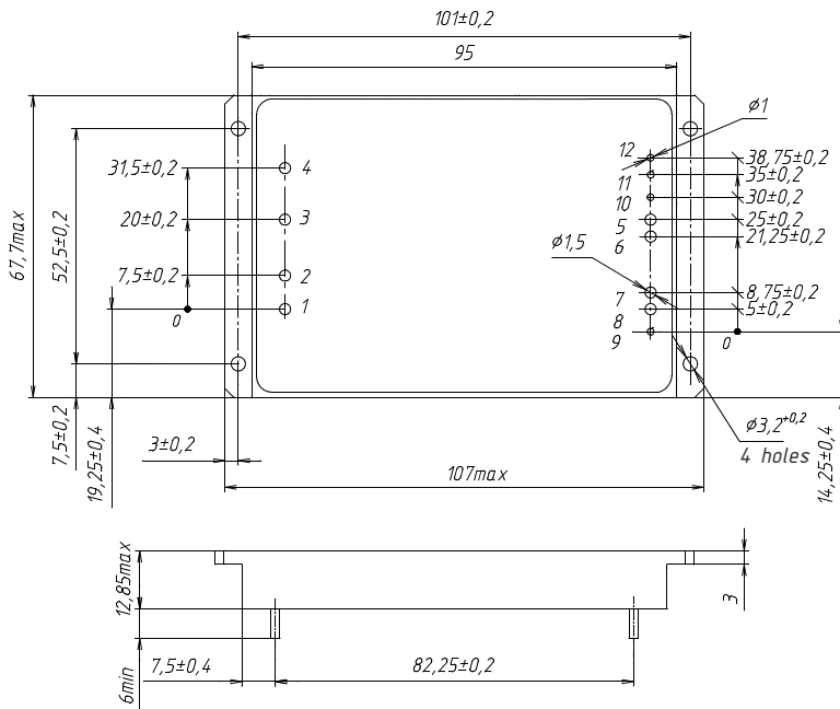
Figure 9. Single-output models.
