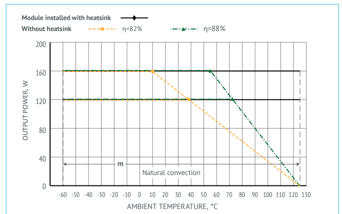
Figure 6 (b). Power derating of MDVm160-xxx.
