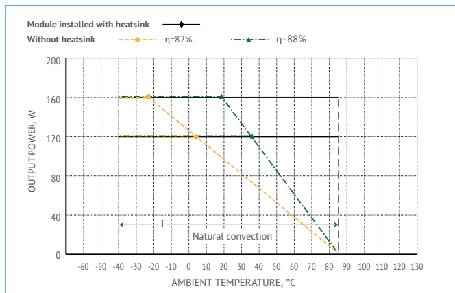
Figure 6 (a). Power derating of MDVi160-xxx.
