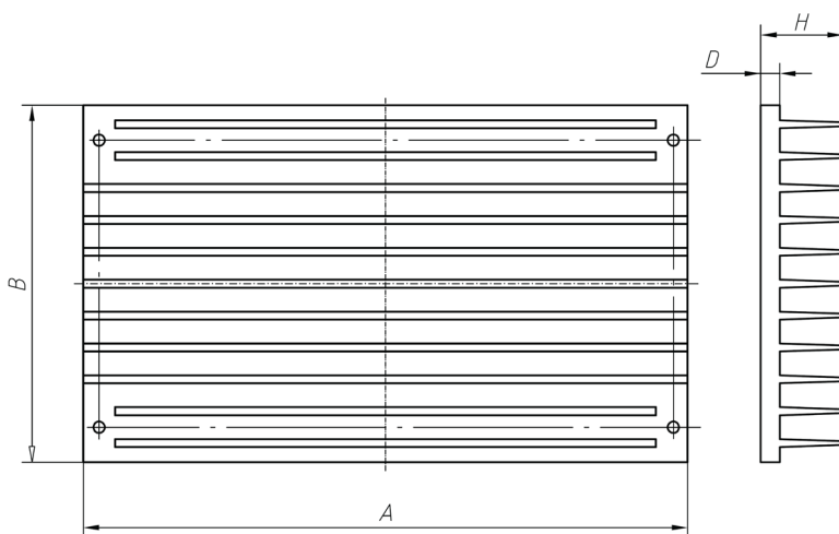
Figure 9. Heatsink with longitudinal ribs 168×125×45×6 mm (A×B×H×D).
