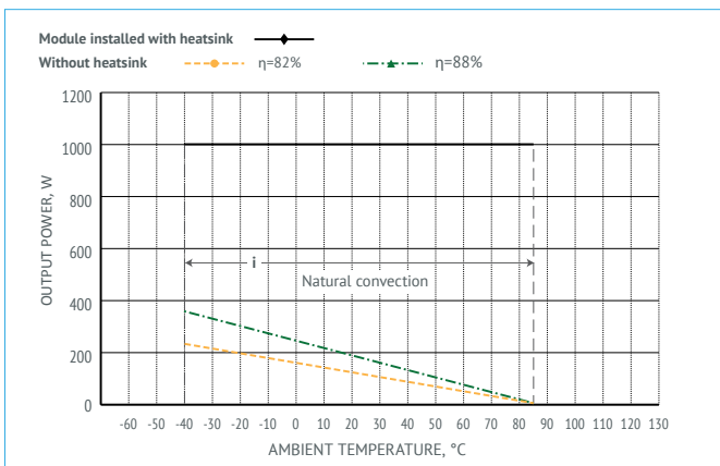
Figure 6 (a). Power derating of MDVi1000-xxx.
