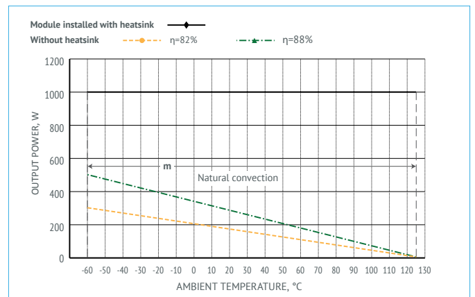
Figure 6 (b). Power derating of MDVm1000-xxx.
