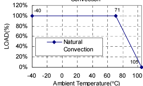
Typical Derating curve for Natural Convection
