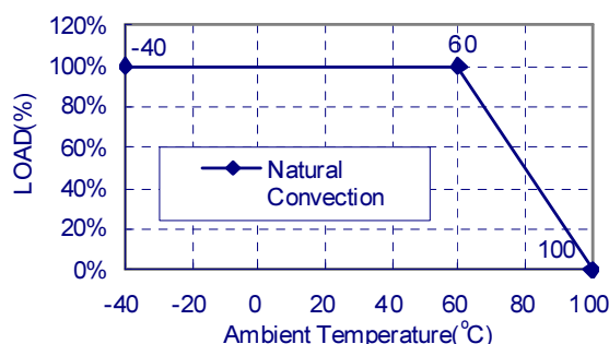
Typical Derating curve for Natural Convection
