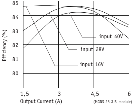
Figure 1 : Typical efficiency versus load at various input
