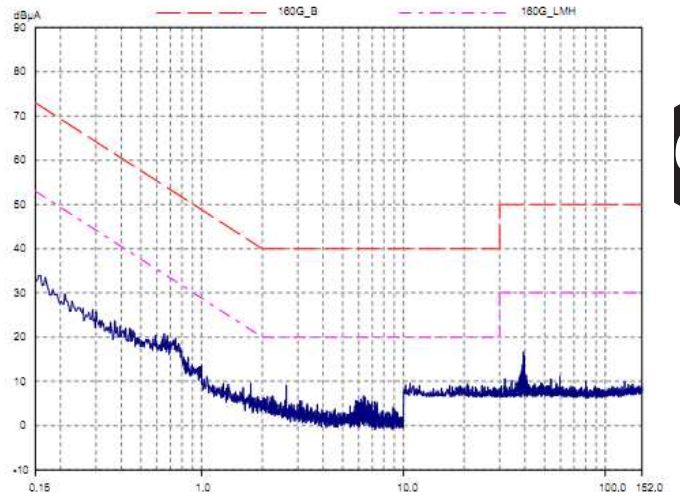
D0-160G : MGDS-150-H-J with FGDS-10A-50V
