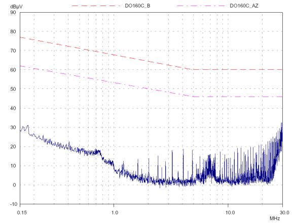
DO-160C : MGDS-75-O-C with FGDS-10A-50V
