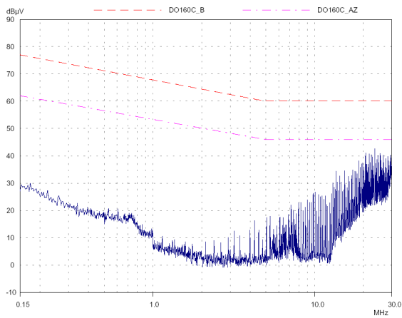
DO-160C : MGDS-100-M-26 with FGDS-10A-50V
