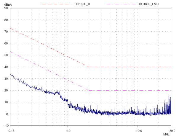
DO-160C : MGDS-150-H-J with FGDS-10A-50V
