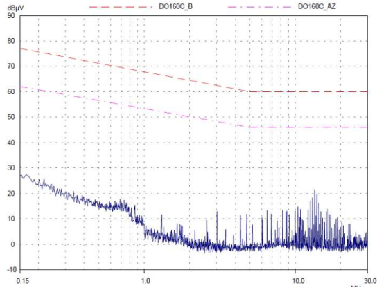
DO-160C : MGDS-75-H-F with FGDS-10A-50V
