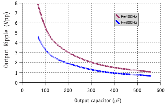
Output Ripple vs Output Capacitor for HGMS-350-W-T
