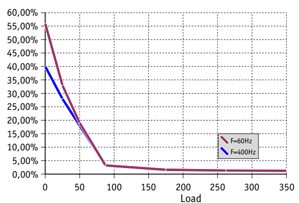
Total Harmonic Distorsion (THD) at 115Vac for HGMS-350-X-T
