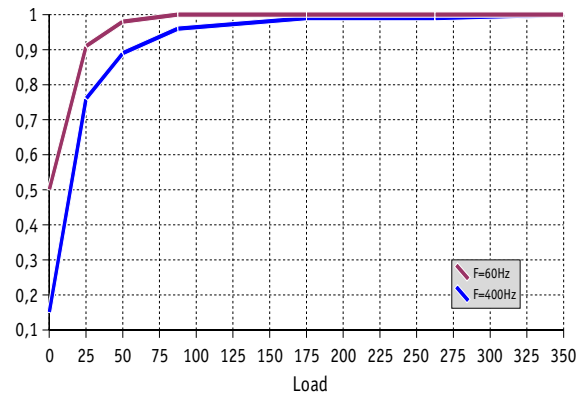
Power Factor (PF) versus Load at 115Vac for HGMS-350-X-T
