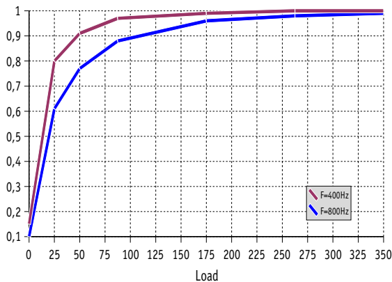
Power Factor (PF) versus Load at 115Vac for HGMS-350-W-T
