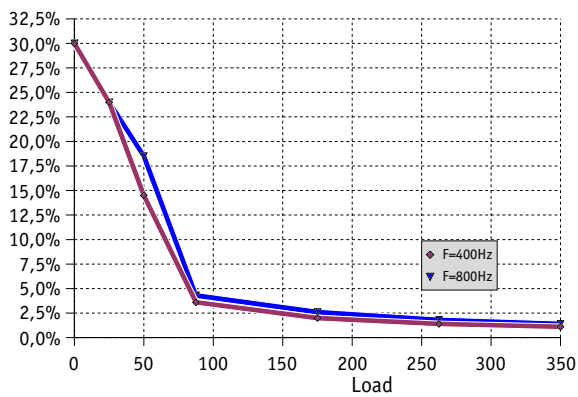
Total Harmonic Distorsion (THD) at 115Vac for HGMS-350-W-T
