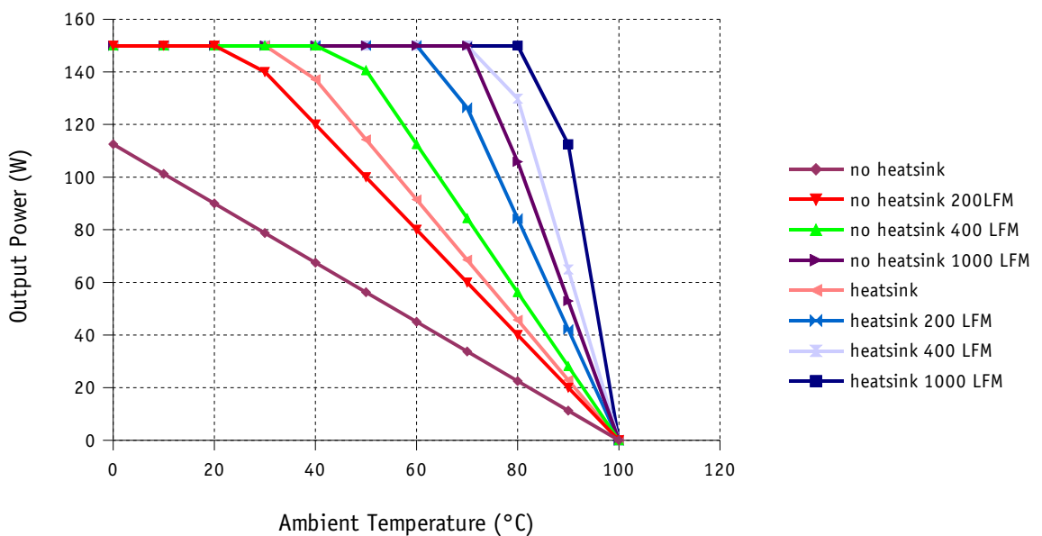
HGMS-150 Thermal Curves
